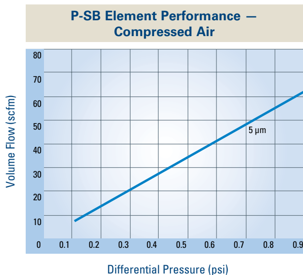
These curves define the flow of a 1030 filter element at standard conditions (14.7 psia; 68°F. R.H.= 70%)
